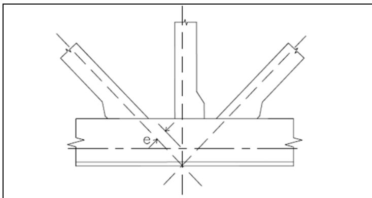
Figure 4.5-1 Single Angle Web Members and Bottom Chord Workpoint Eccentricity
