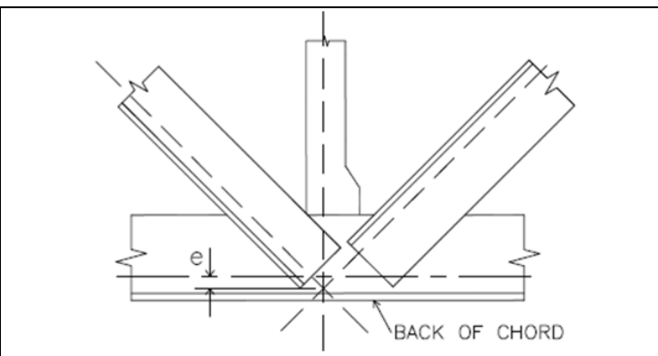
Figure 4.5-2 Multiple Web Members and Bottom Chord Workpoint Eccentricity
