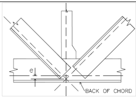
Figure 4.5-2 Multiple Web Members and Bottom Chord Work Point Eccentricity
